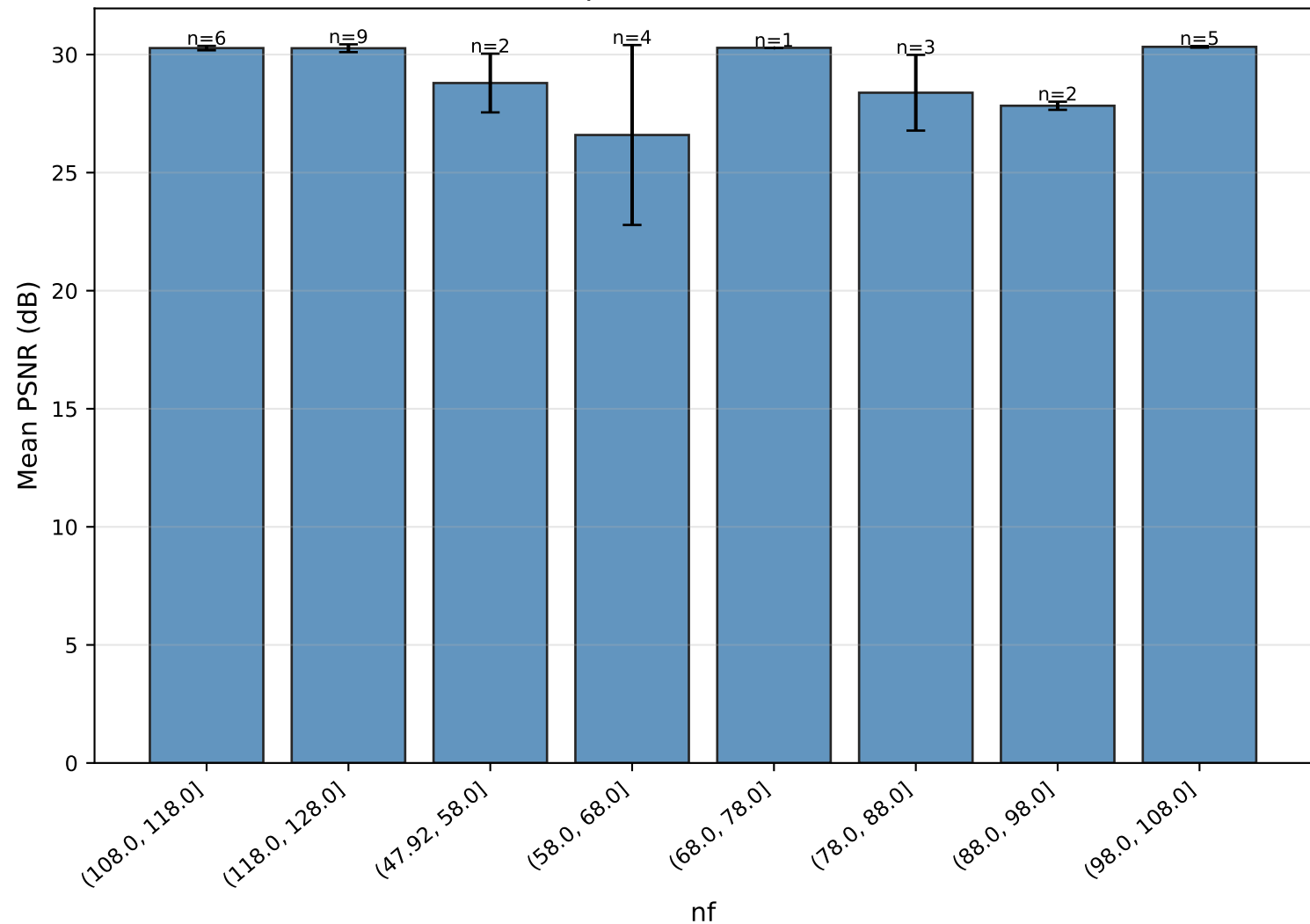
Mean PSNR per value of nf — SRFormer
